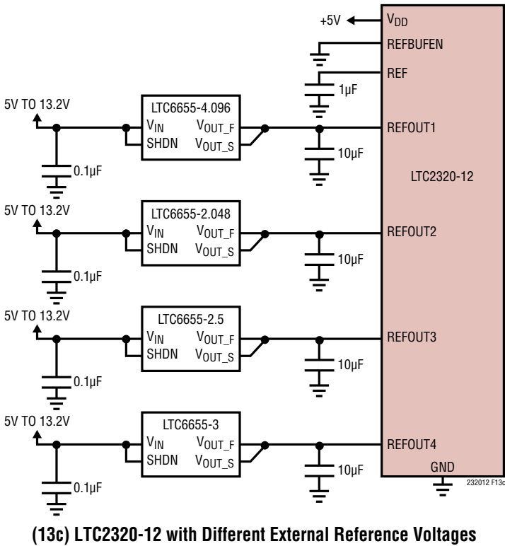
Figure 13. Reference Connections
