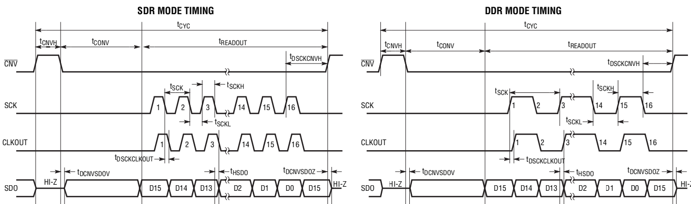
Figure 21. LTC2320-12 Timing Diagram
